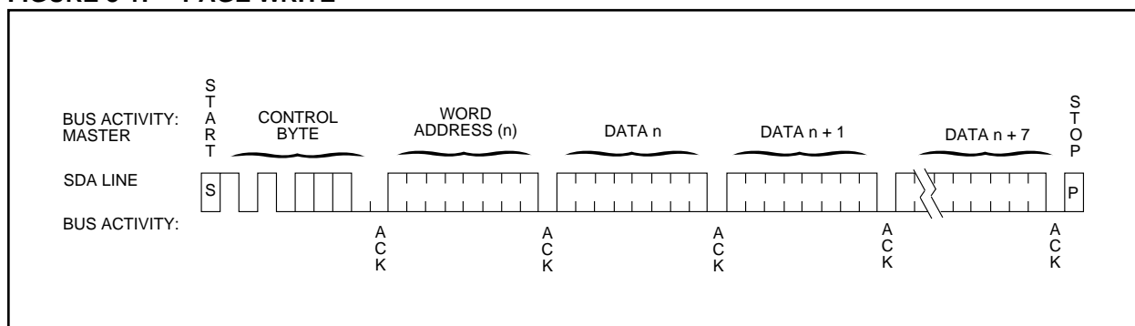
FIGURE 8-1: PAGE WRITE
