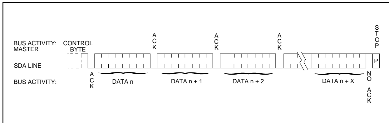
FIGURE 9-1: SEQUENTIAL READ
