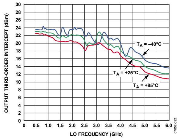
Figure 43. OIP3 vs. LO Frequency ( f_{LO} ) and Temperature ( P_{OUT} = -5 dBm @ f_{LO} = 900 MHz)
