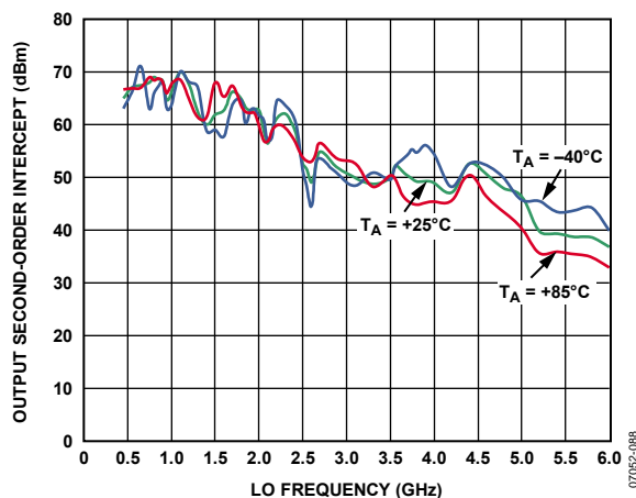
Figure 19. OIP2 vs. LO Frequency ( f_{LO} ) and Temperature ( P_{OUT} = -5 dBm @ f_{LO} = 900 MHz)
