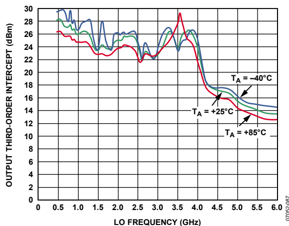
Figure 18. OIP3 vs. LO Frequency ( f_{LO} ) and Temperature ( P_{OUT} = -5 dBm @ f_{LO} = 900 MHz)
