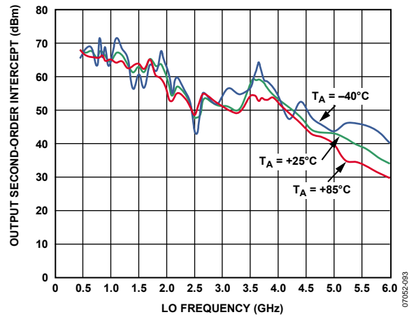
Figure 44. OIP2 vs. LO Frequency ( f_{LO} ) and Temperature ( P_{OUT} = -5 dBm @ f_{LO} = 900 MHz)
