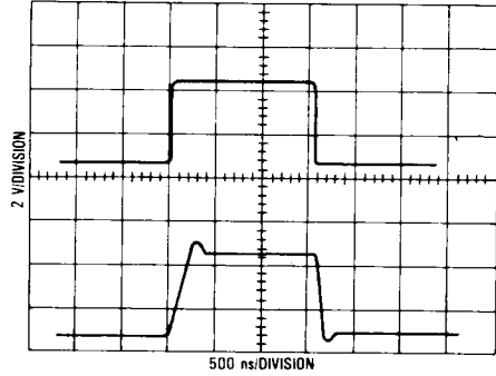
LARGE SIGNAL TRANSIENT RESPONSE V_{DD} = 10\text{ V} NON-INVERTING UNITY GAIN I_{Set} = 200\ \mu\text{A} , V_{in} AVERAGE = 5 V
