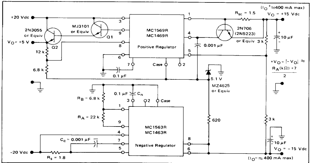
FIGURE 29 — \pm 15\text{ Vdc} COMPLEMENTARY TRACKING REGULATOR WITH AUXILIARY +5.0\text{ V} SUPPLY
