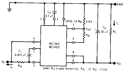
FIGURE 6 - LOAD REGULATION
