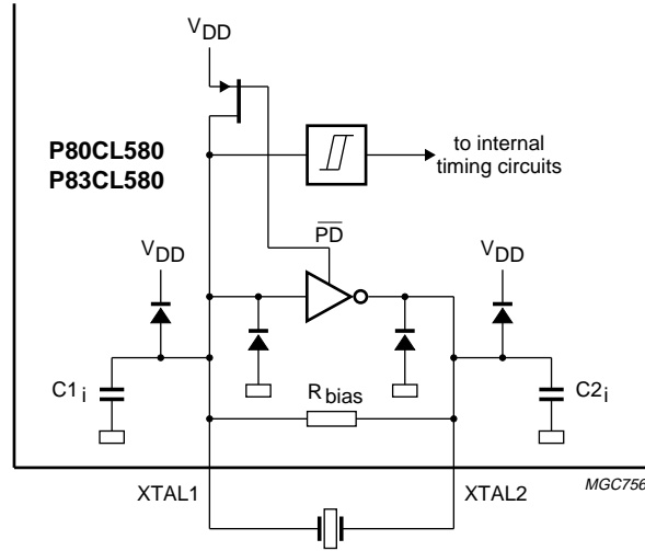
Fig.29 Standard oscillator.
