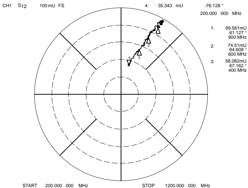
Figure 6. LNA Transmission and Isolation Characteristics (at Device Pin)
