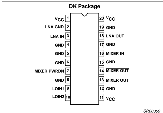
Figure 1. Pin Configuration
