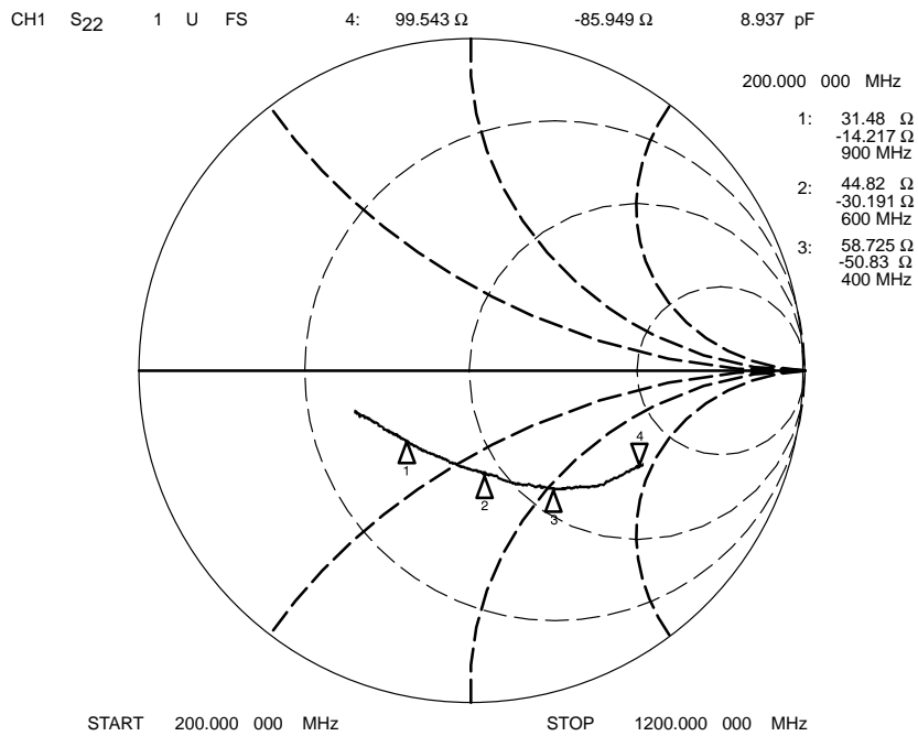
Figure 5. LNA Input and Output Match (at Device Pin)
