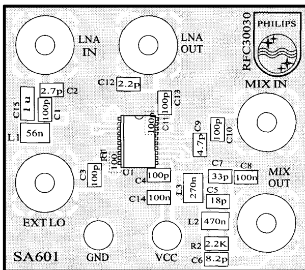
Silk Screen
