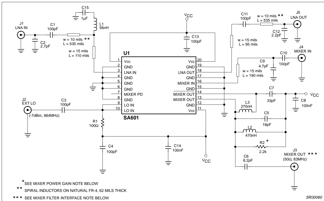
Figure 3. Application Circuit
