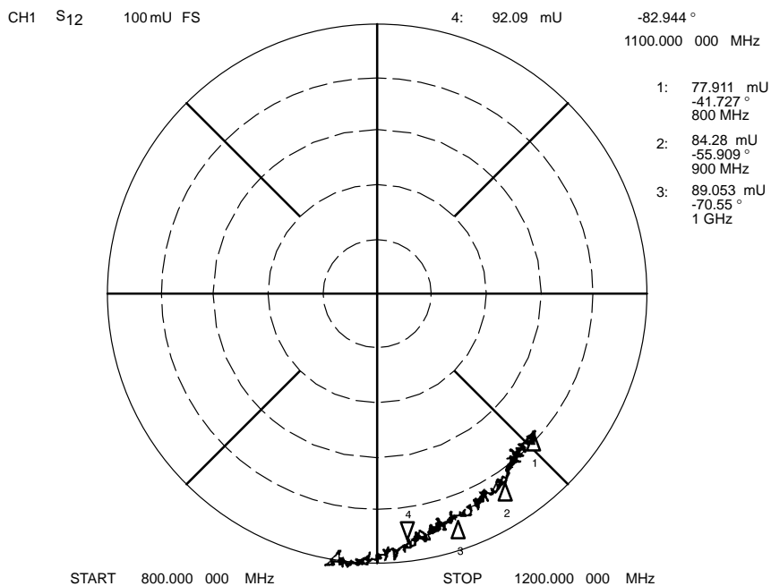
Figure 5. LNA Transmission and Isolation Characteristics (at Device Pin)
