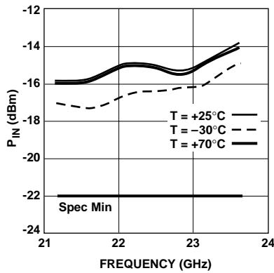
Figure 4. Power In at P_{1dB} Out vs. Frequency.
