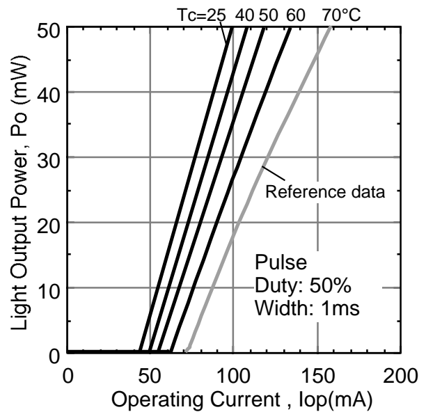
Light Output Power vs. Current (Pulse)
