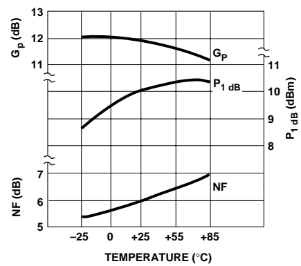
Figure 3. Output Power at 1 dB Gain Compression, NF and Power Gain vs. Case Temperature, f = 1.0 \text{ GHz} , I_d = 35 \text{ mA} .
